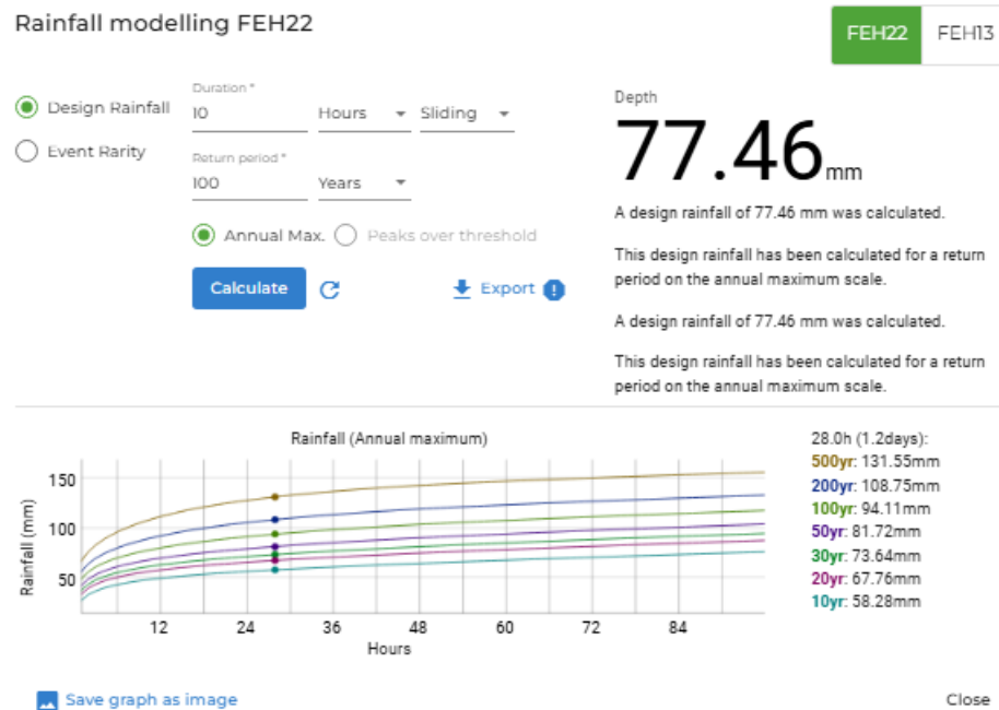
Figure 5.1 – Depth-Duration Frequency 1%AEP 10 hour duration storm
